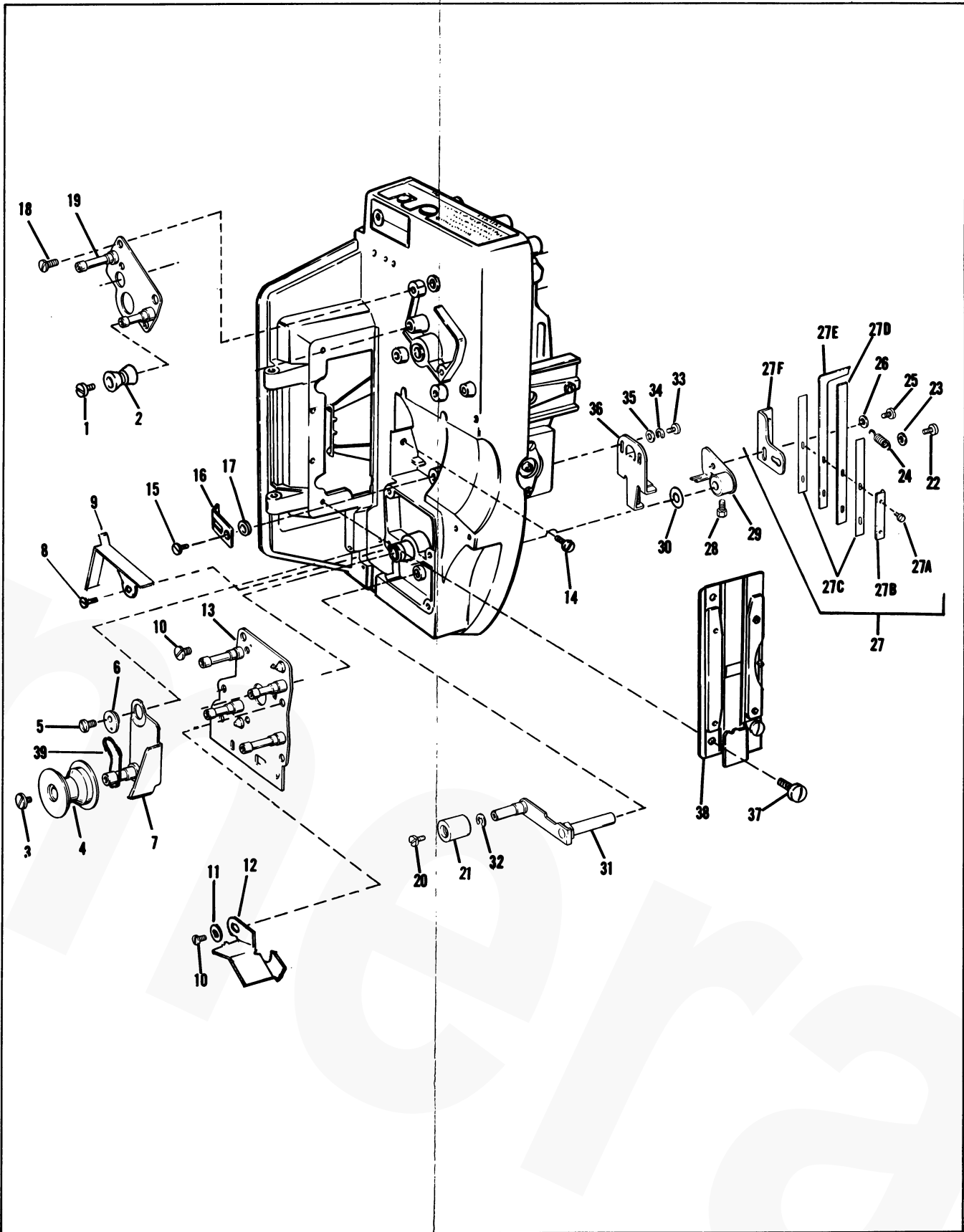
Figure 10. Mechanism Assembly (Continued)
