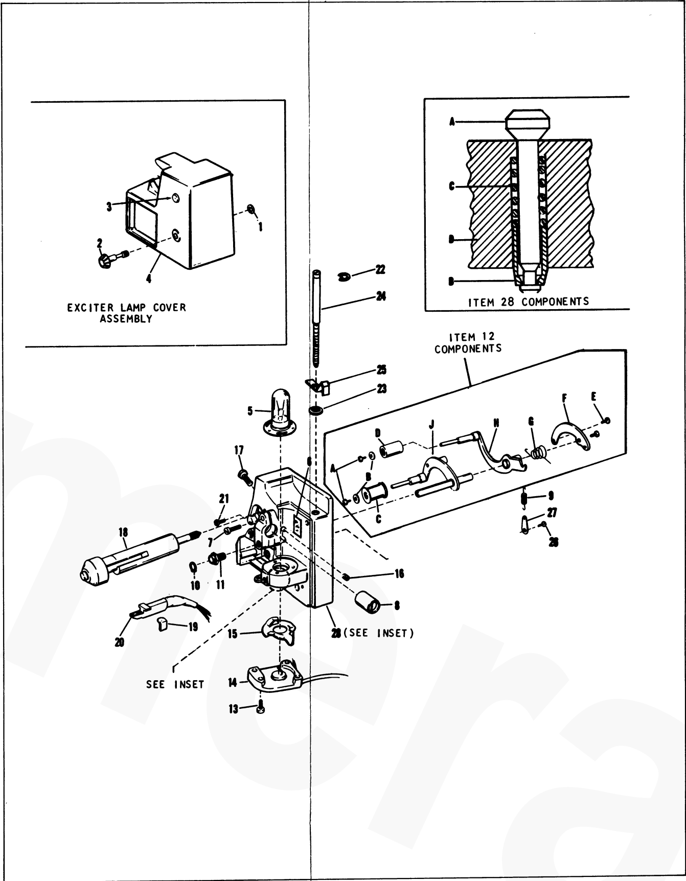
Figure 8. Exciter Lamp Cover and Soundhead
