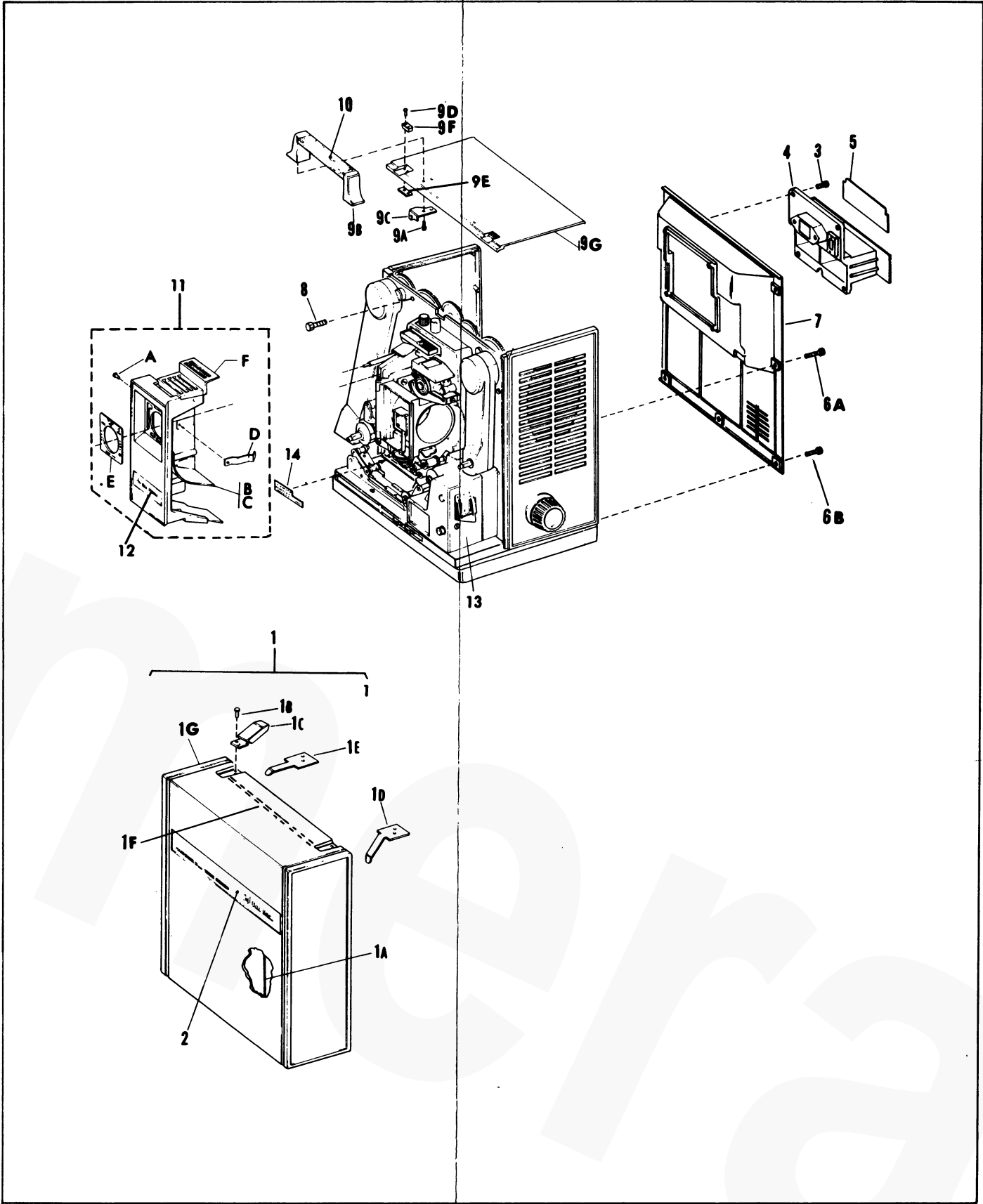
Figure 1. Covers and Lamphouse
