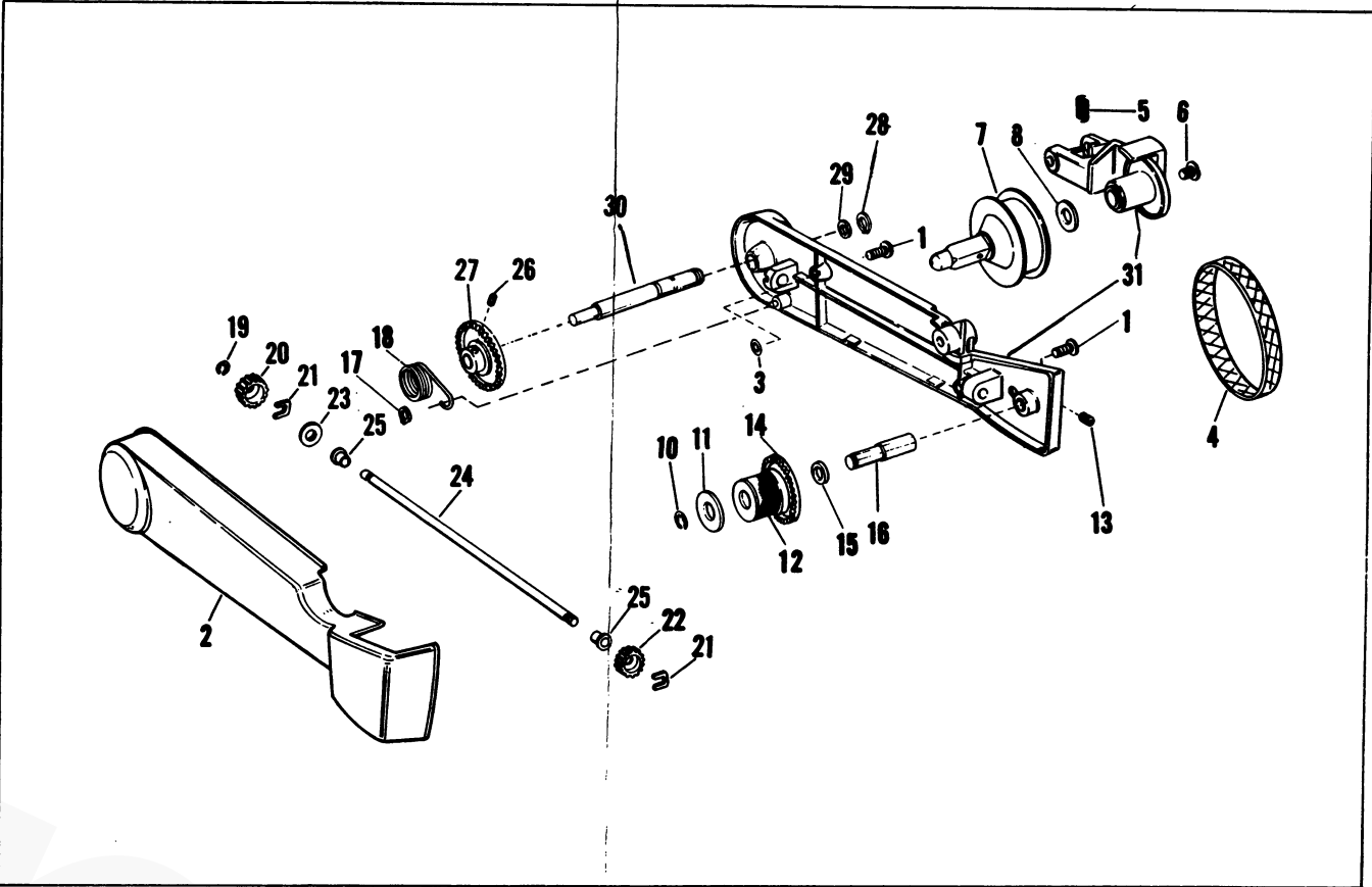
Figure 7. Rear Reel Arm Assembly
