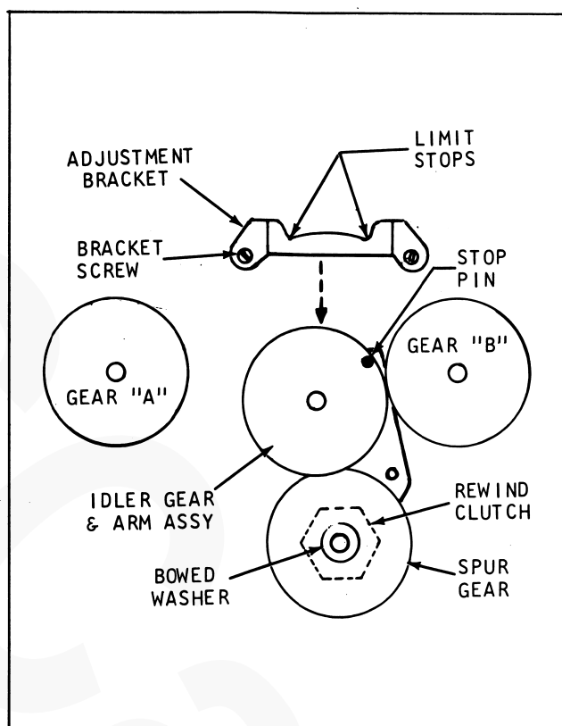
Figure N. Adjusting Gear Shift Tension and Backlash
