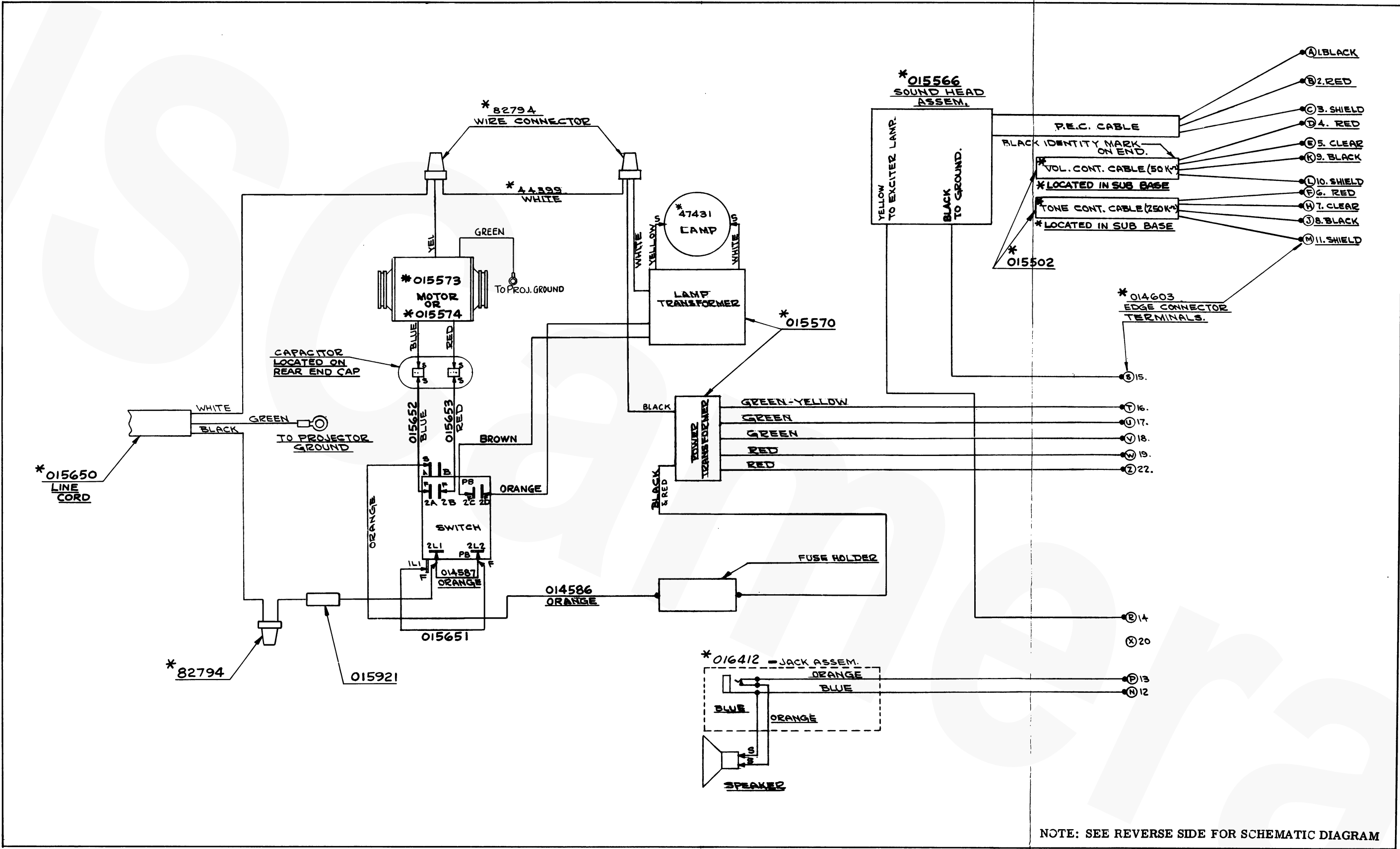
Figure 14. Projector/Amplifier Wiring Diagram (Model 1574C)
