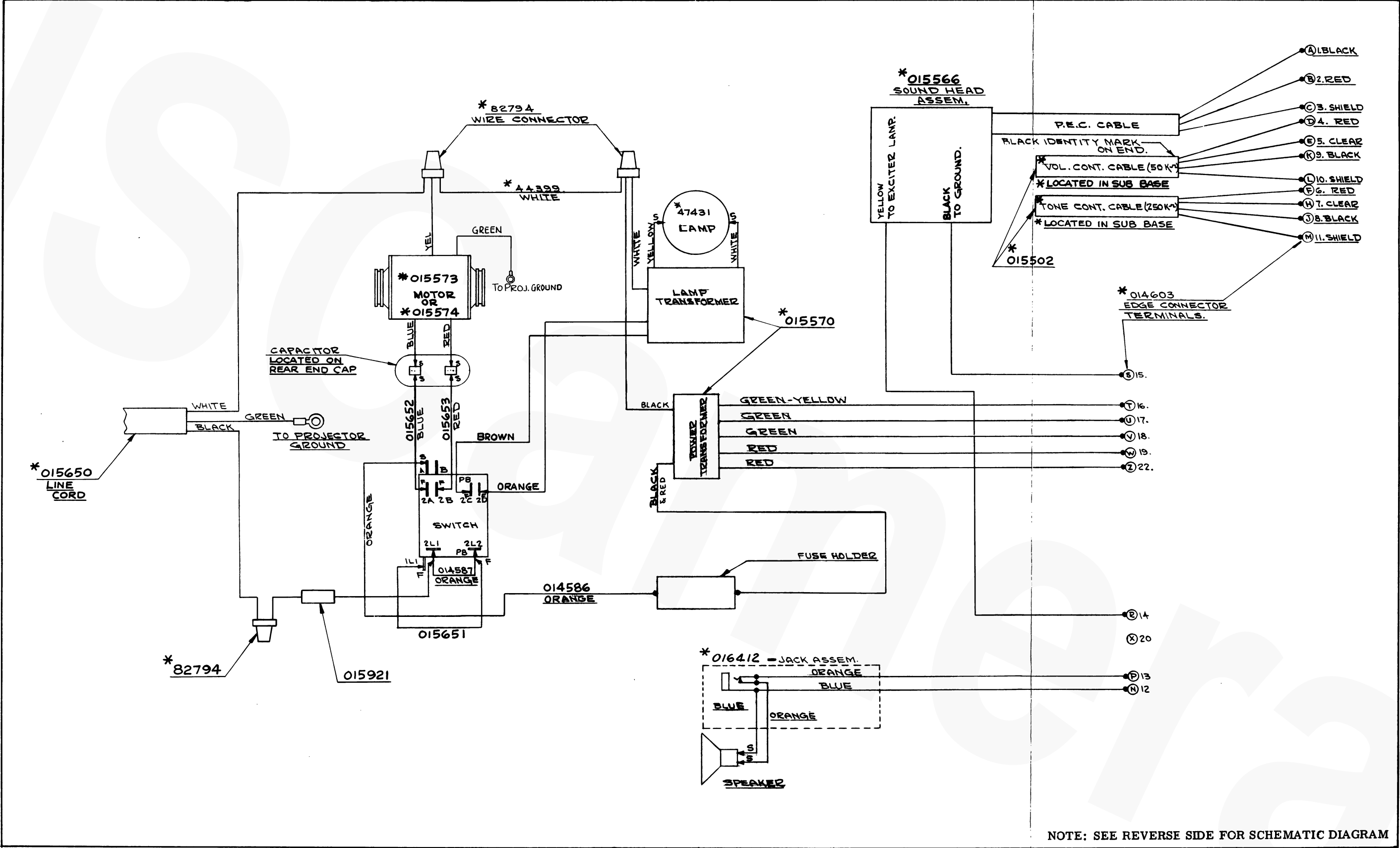
Figure 15. Projector/Amplifier Wiring Diagram (Models 1579C/1579CS)
