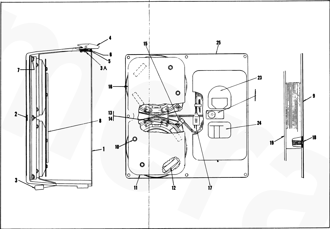
Figure 13. Front Speaker/Cover Assembly (P/N 016507) (Model 1579CS Only)
