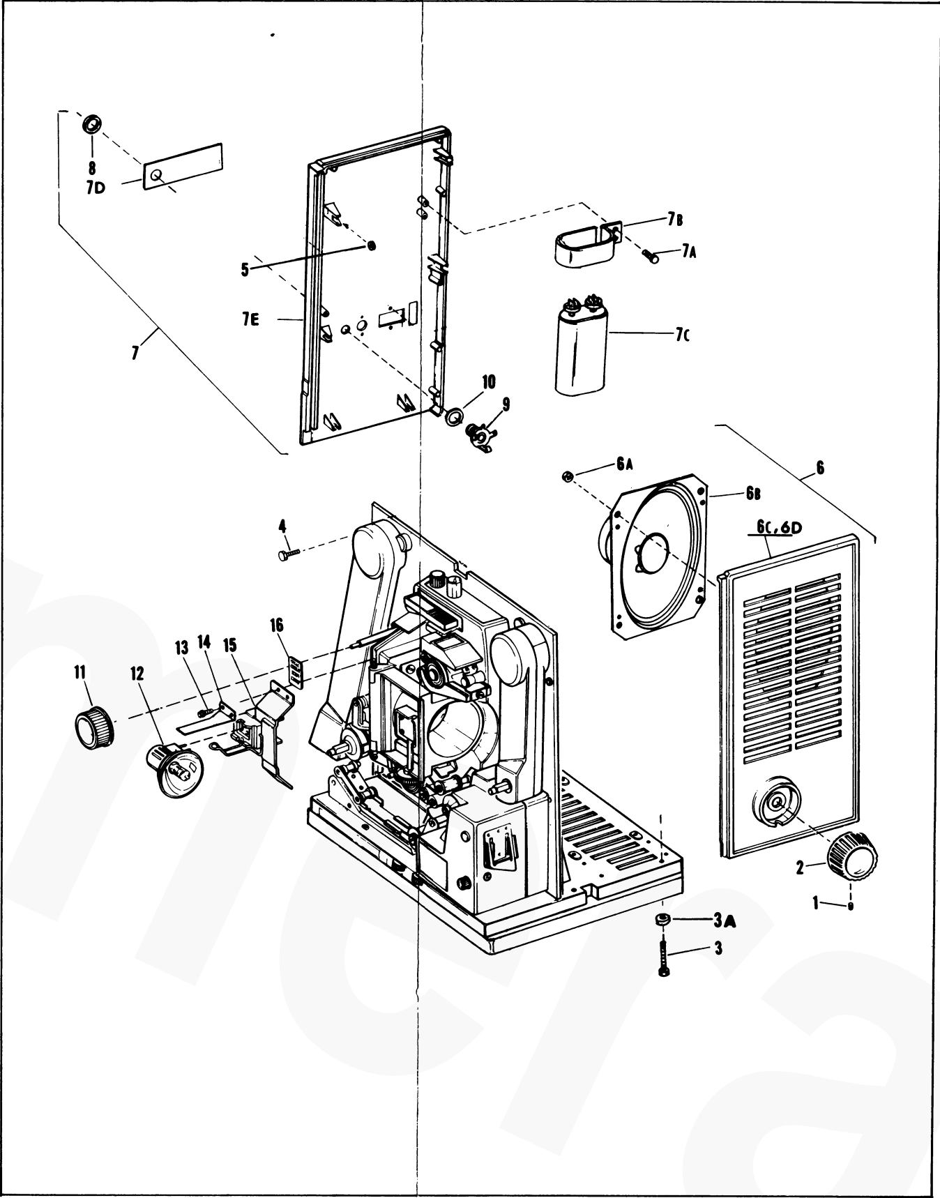
Figure 2. End Caps and Lamp Parts
