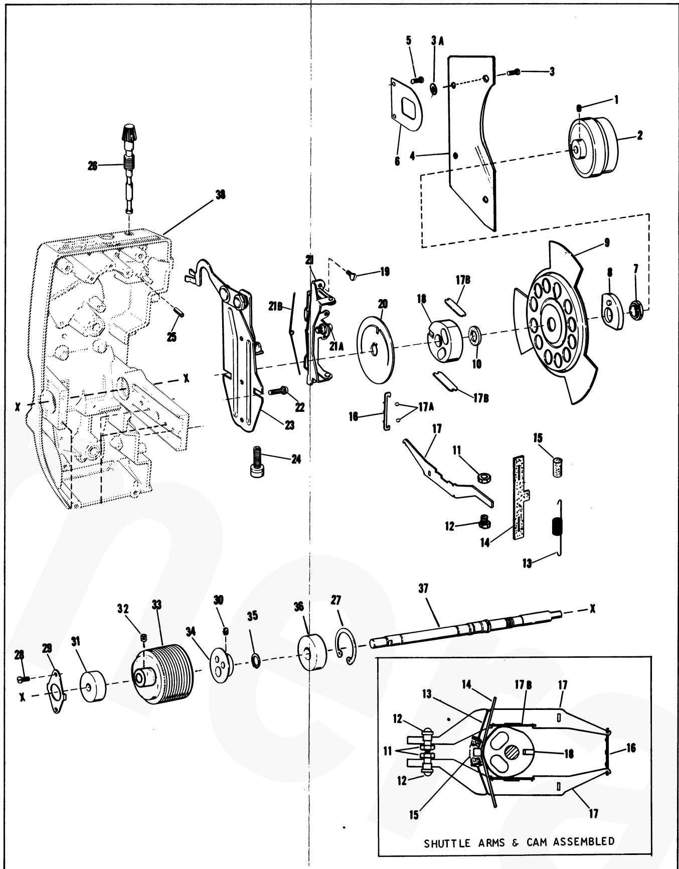
Figure 11. Mechanism Assembly (Continued)
