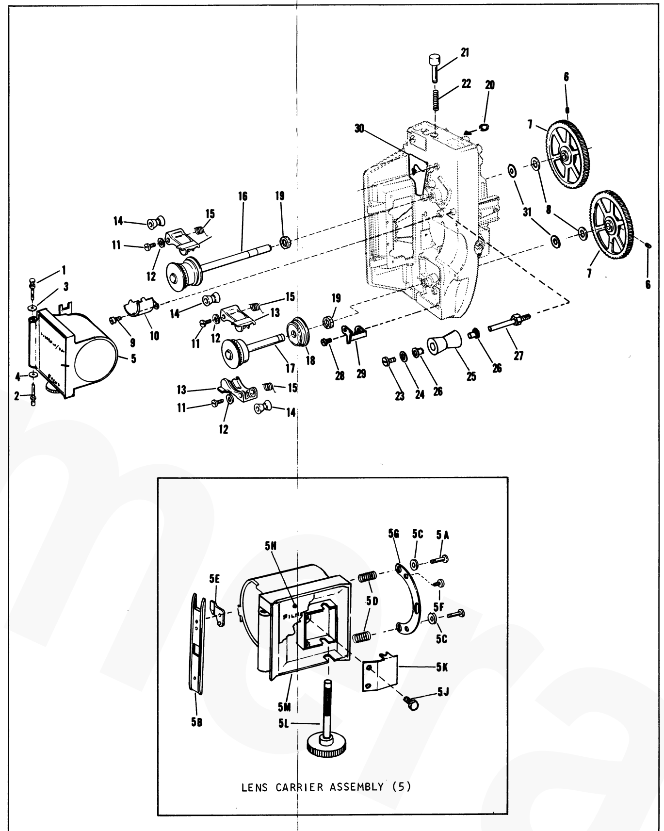
Figure 9. Mechanism Assembly
