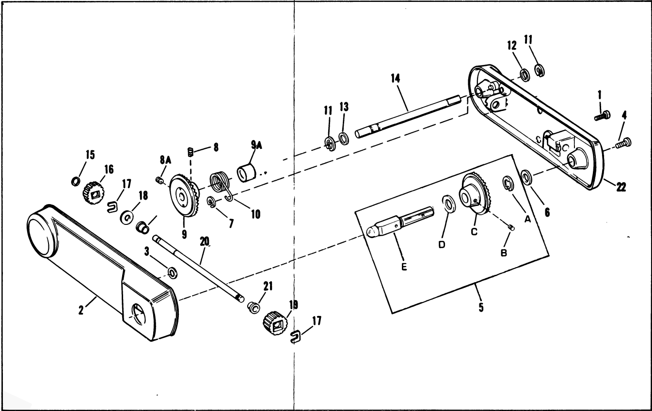
Figure 6. Front Reel Arm Assembly
