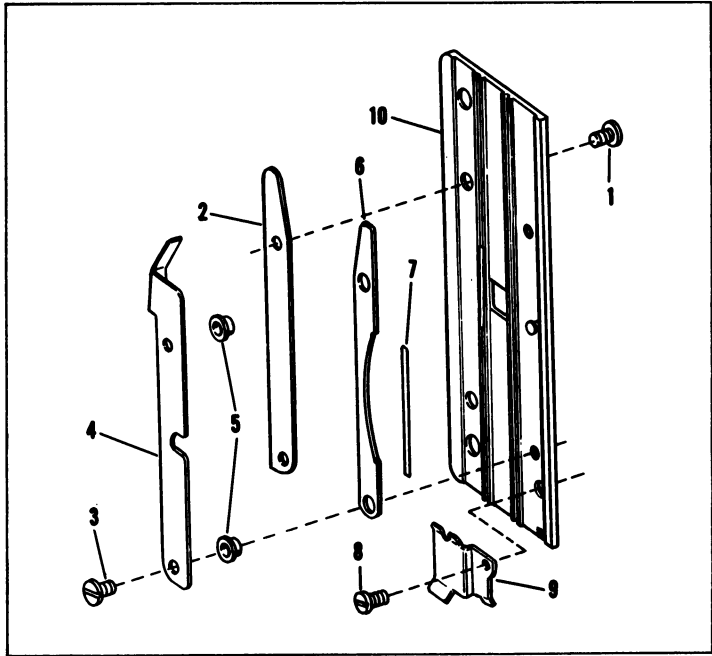
Figure 12. Aperture Plate Assembly
