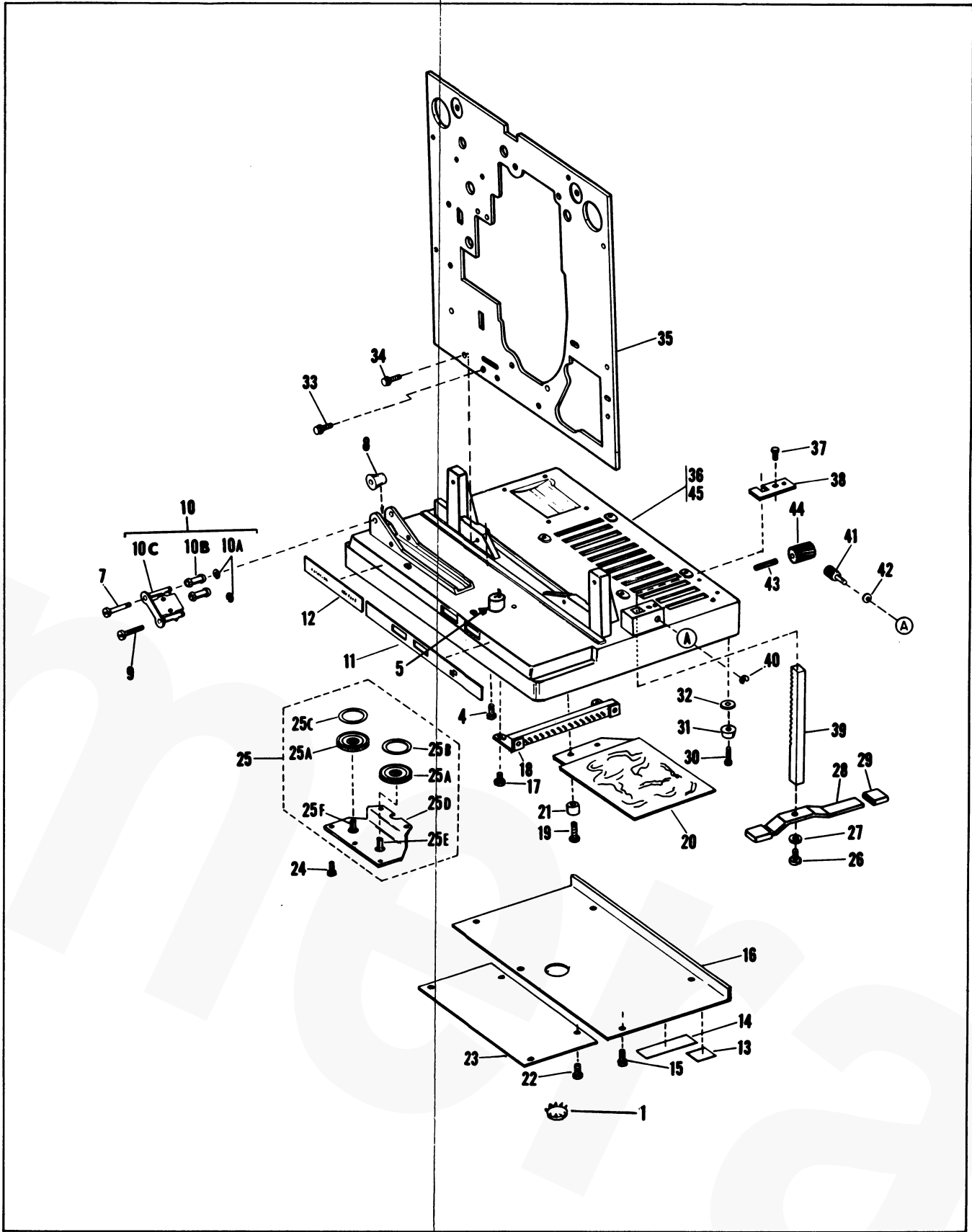
Figure 5. Mainplate and Base Components
