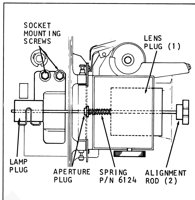
Figure E. Aligning the Optical System
