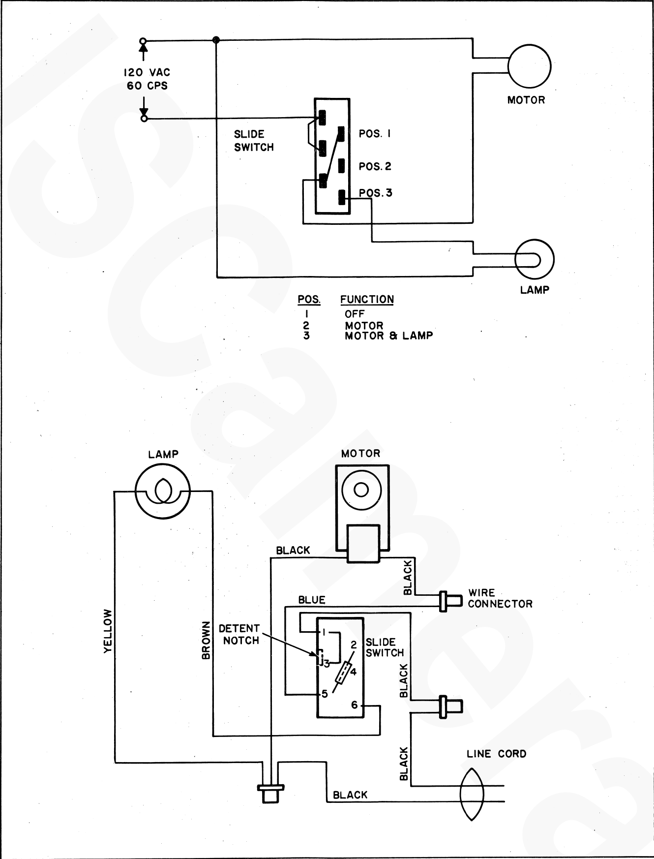
Figure 8. Schematic and Wiring Diagrams
